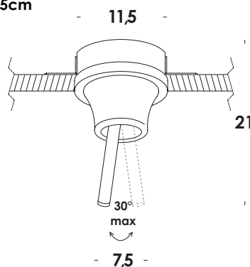
CONICAL DIAGRAM
