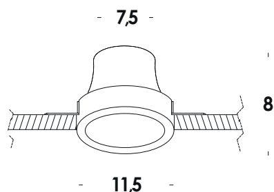
CONICAL DIAGRAM
