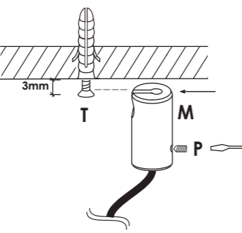
fig.2 - acc. terminale cavo acc. terminal for cable
