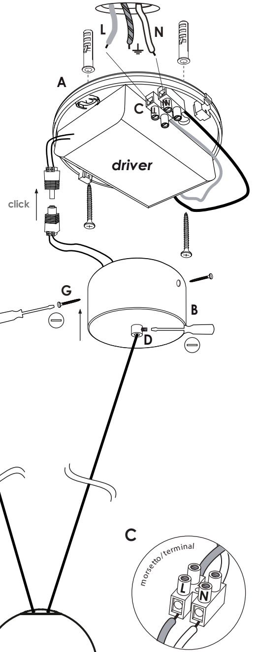
fig.2 - acc. terminale cavo acc. terminal for cable
