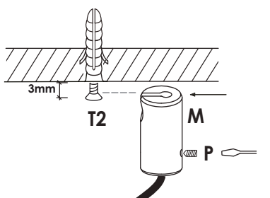
fig.2 - acc. terminale cavo acc. terminal for cable
