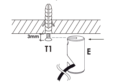
fig.1 - acc. passante cavo acc. open for cable
